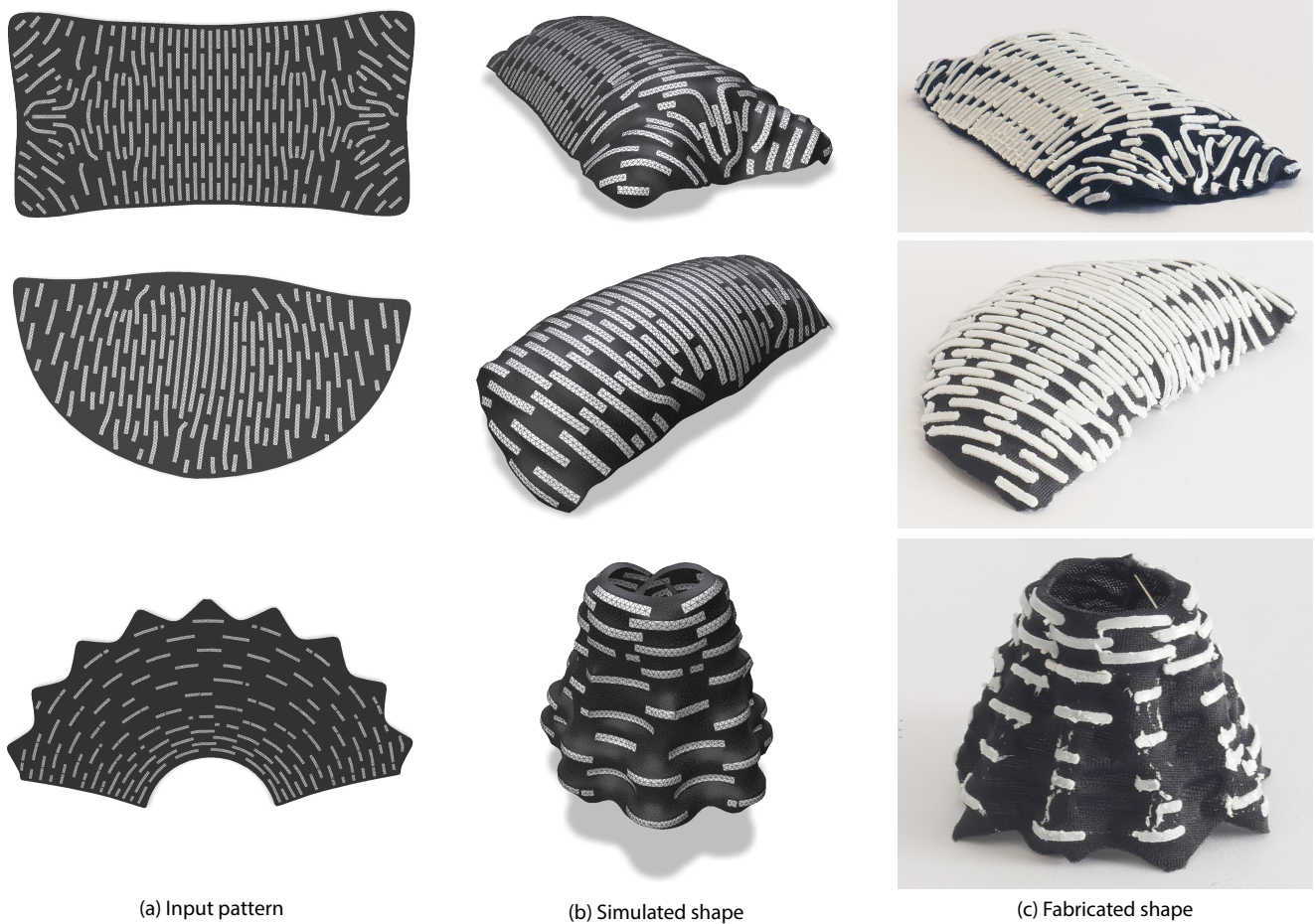
Figure 13: Visual comparison between the results of our simulator (b) and fabricated assemblies (c), using patterns computed with the inverse-design method of Jourdan et al. [2022] (a). The Skirt pattern (bottom row) contains strips printed on the back side of the fabric to produce negative extrinsic curvature.
